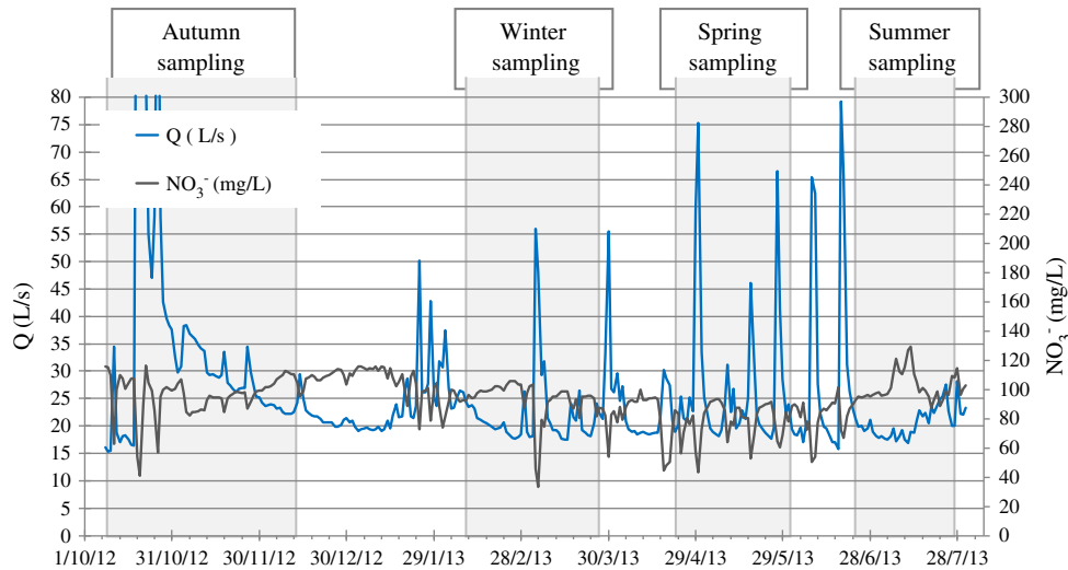
Fig. 2. Flow and nitrate concentration were registered with an in-situ monitoring system; data plotted are daily averages provided by IGME Institute. The gray-shadowed blocks are the colonization periods of the algal biofilm on the artificial substrata.
