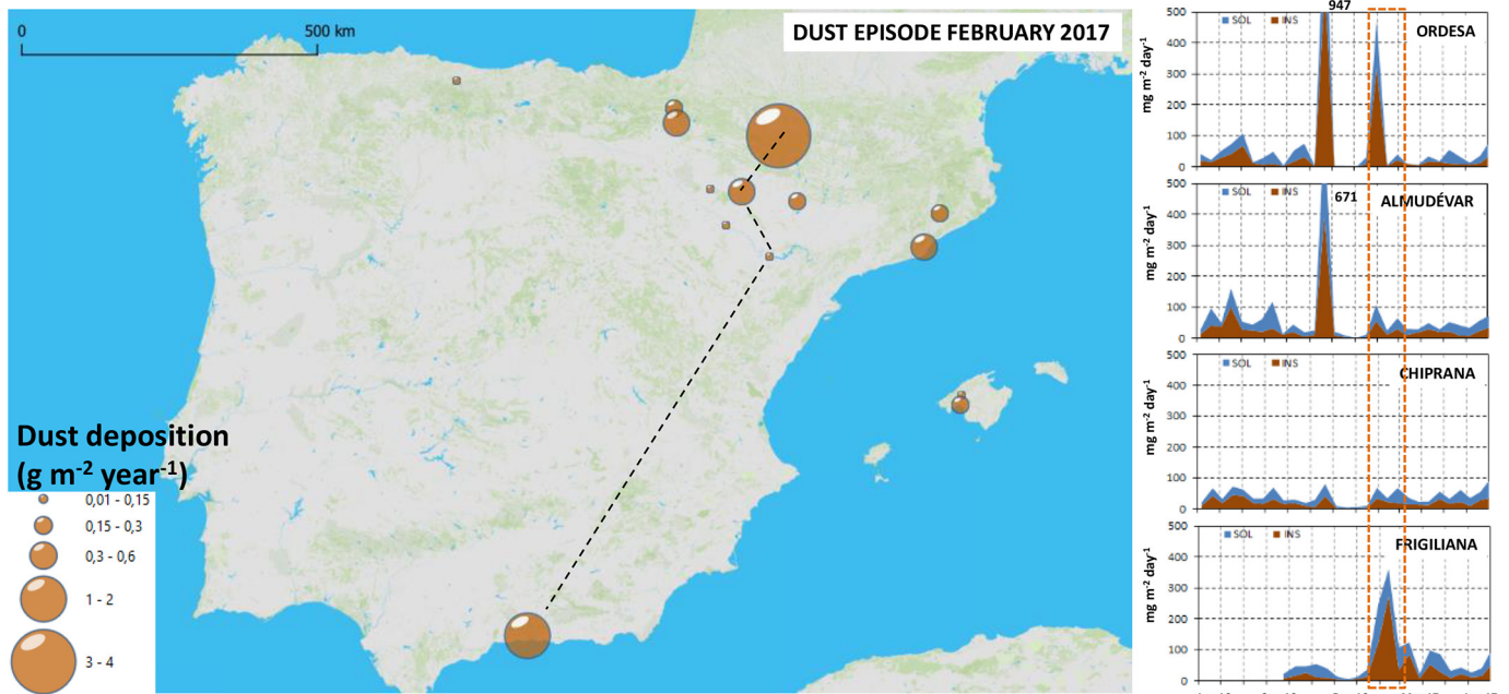
Fig. 8. Left: map showing the annual contribution to DF_{INS} (in g\ m^{-2}\ year^{-1} ) registered in the DONAIRE network as a result of the February 2017 dust event. Right: northern-southern transect illustrating DF_{SOL} and DF_{INS} (in mg\ m^{-2}\ day^{-1} ) recorded at these four sites, illustrating the severity of the February 2017 event in Ordesa and Frigiliana. Note also the impact of the November 2016 episodes in Ordesa and Almudévar.
